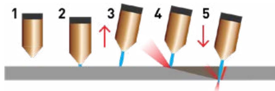
The 5 steps of angled piercing with plasma.
