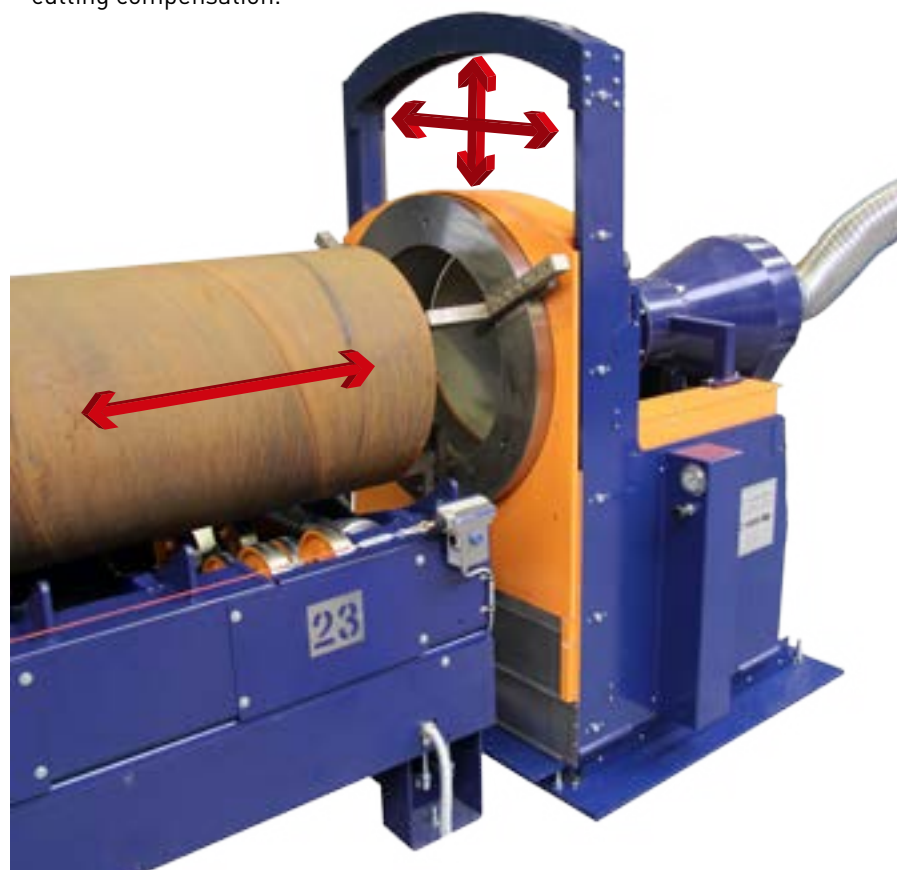
Compensation for pipe deformation of the main drive (SPC 1200 RB version)
