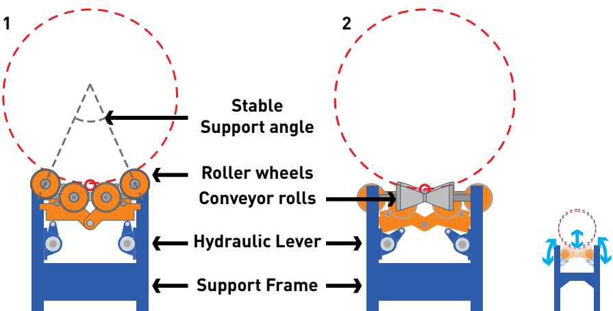
Overview of roller bed components 1. Rotation mode 2. Transport mode
