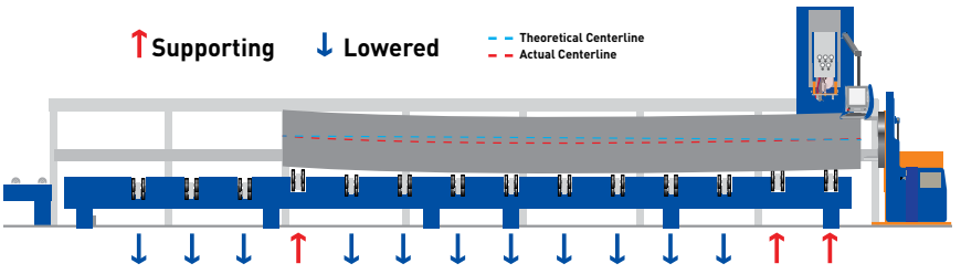
Supporting the pipe on a few positions to correct for bow shapes.
