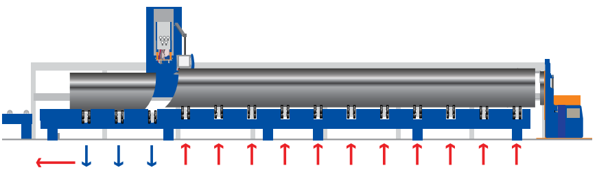
Lowering a few roller beds to feed out small parts that are already cut.
