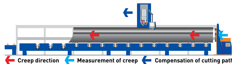
Creep compensation
